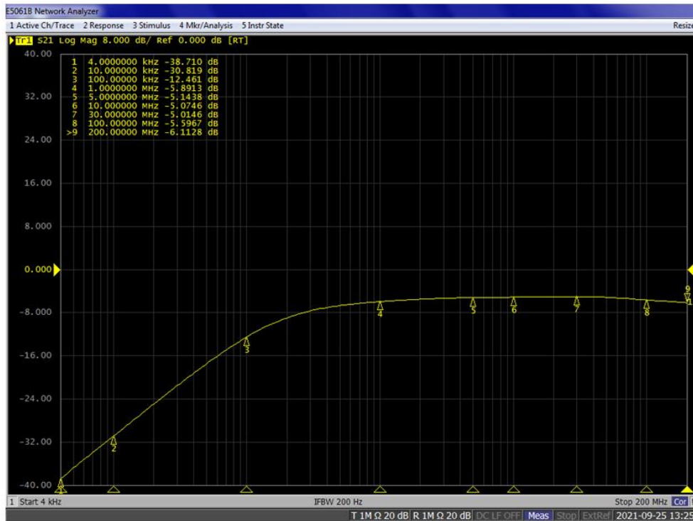
BCIP-200 current injection clamp insertion loss curve
